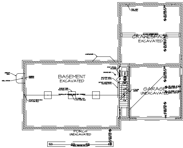
FOUNDATION PLAN SCALE: 1/4"=1'-0"
