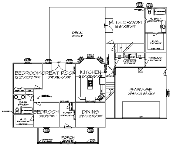
FIRST FLOOR PLAN SCALE: 1/4"=1'-0"
